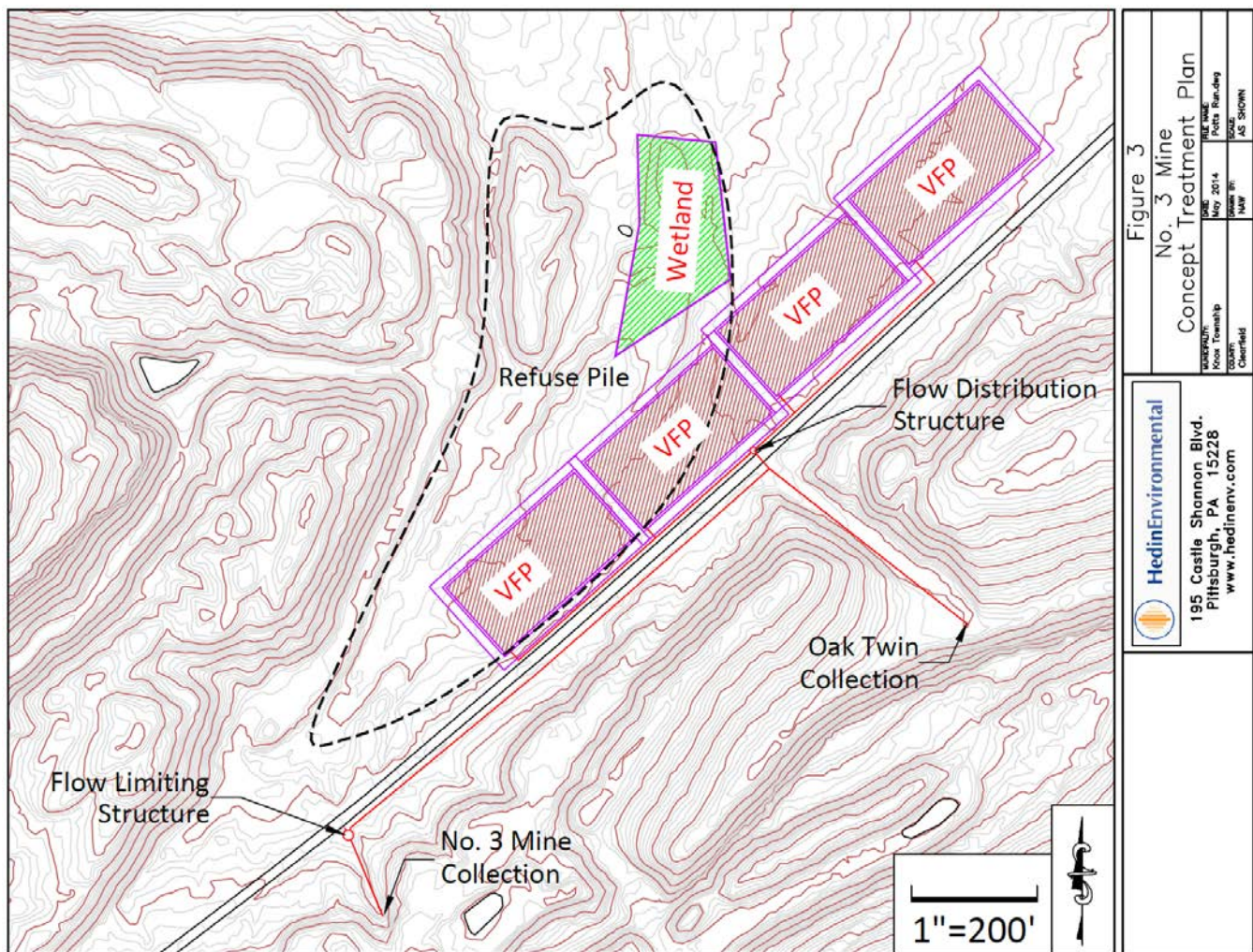
Figure 3. Concept layout for a passive treatment system sized according to Table 11.
